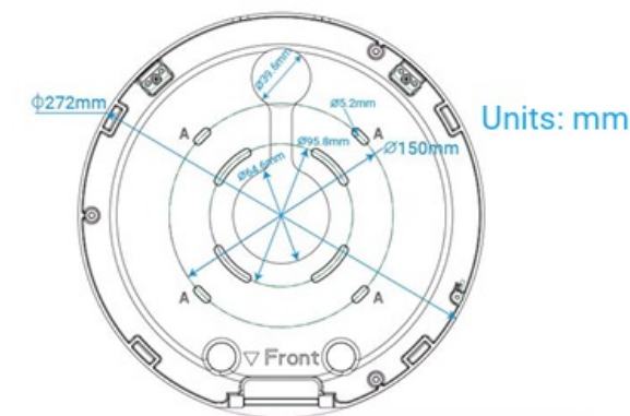
AI Multi-directional Network Camera | Dimensions
