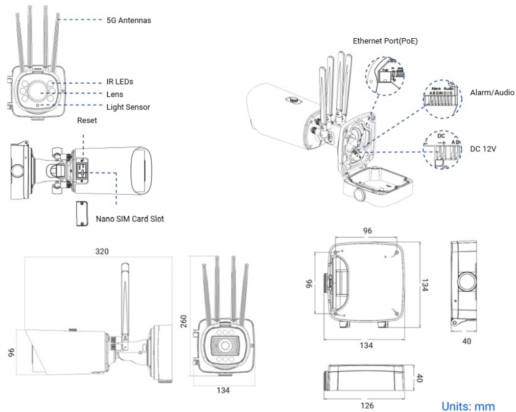
5G AIoT 4X Pro Bullet Plus Network Camera | Dimensions
