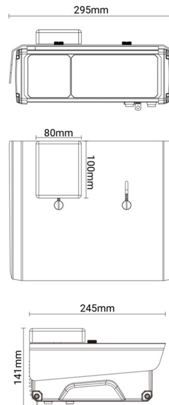
Single Vision TrafficX Camera | Dimensions
