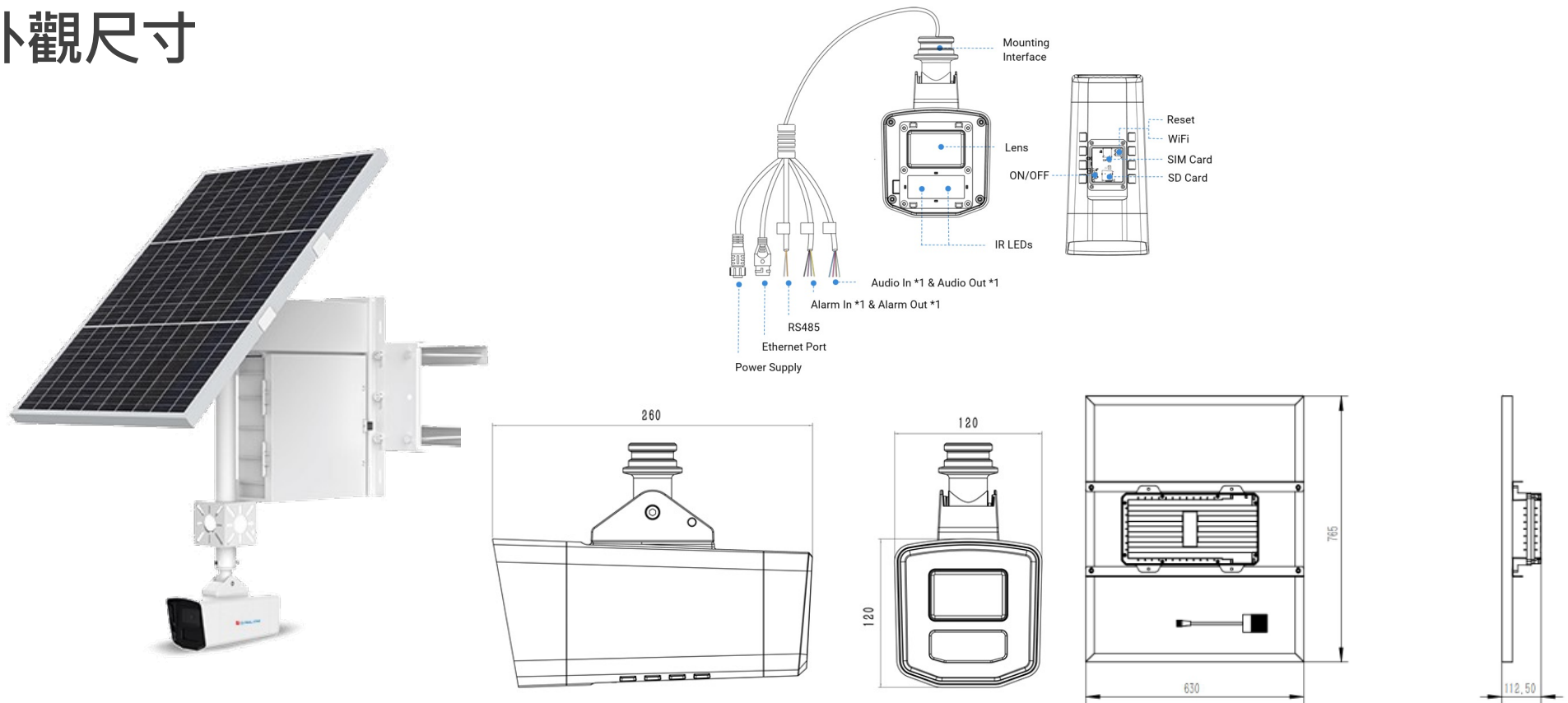
4G Solar-powered Security Camera | Dimensions
