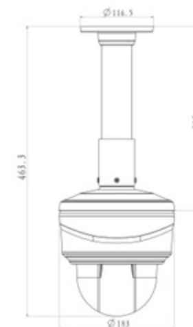
AI 23X PTZ Dome Network Camera | Dimensions
