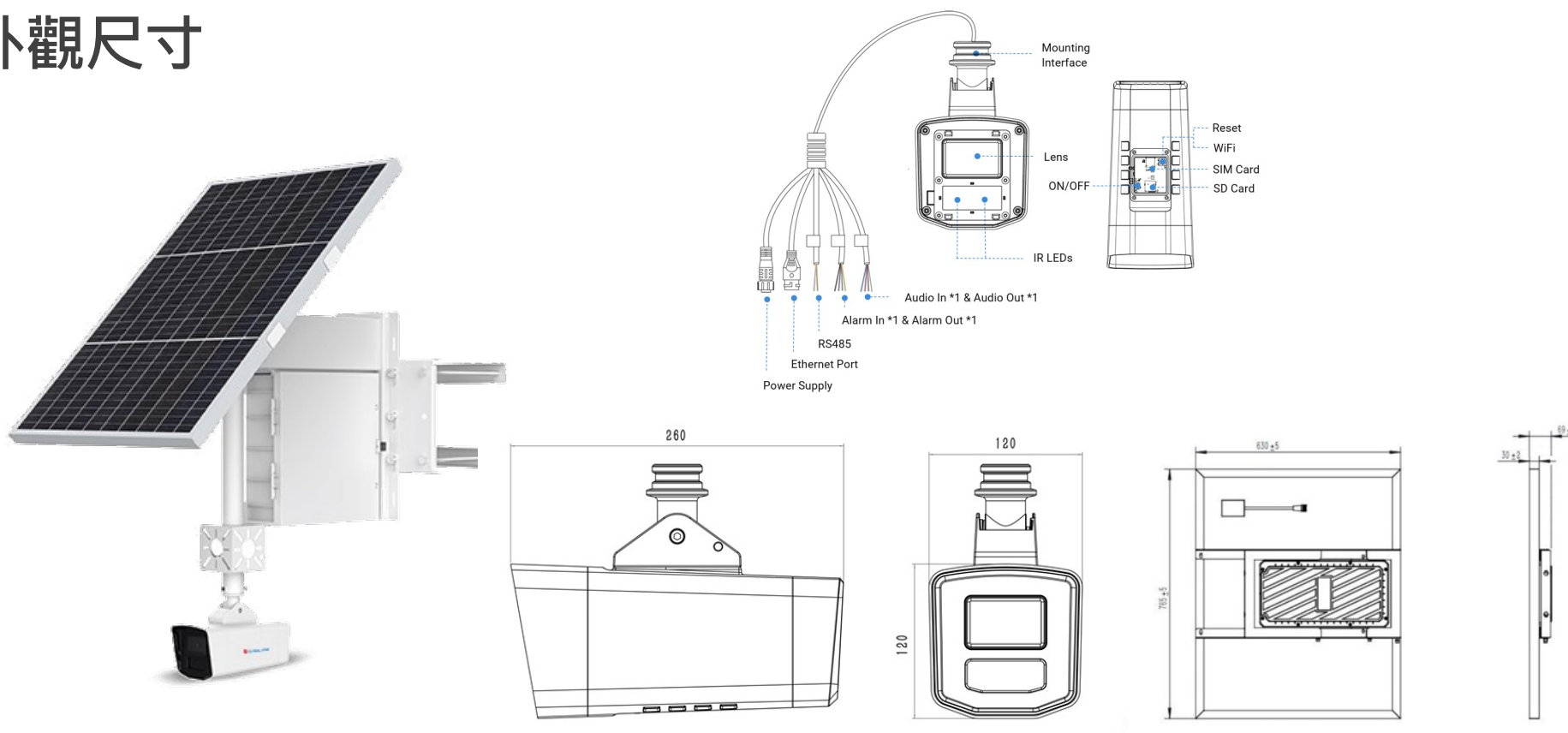
4G Solar-powered Security Camera | Dimensions
