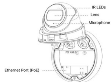
Junction Box Version
