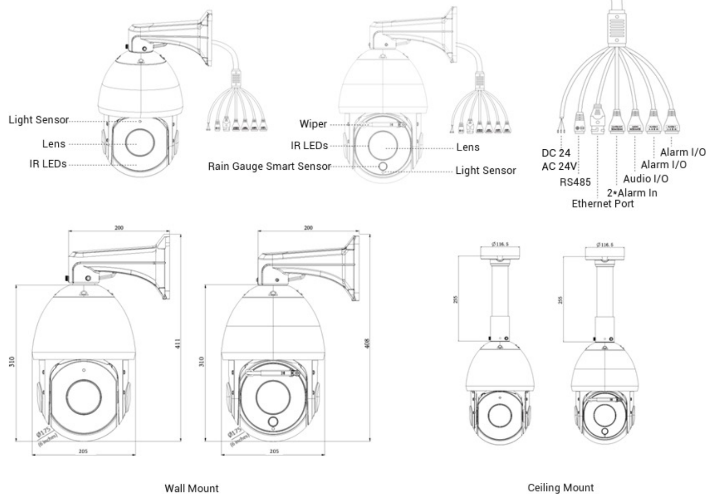
AI 42X Speed Dome Network Camera | Dimensions
