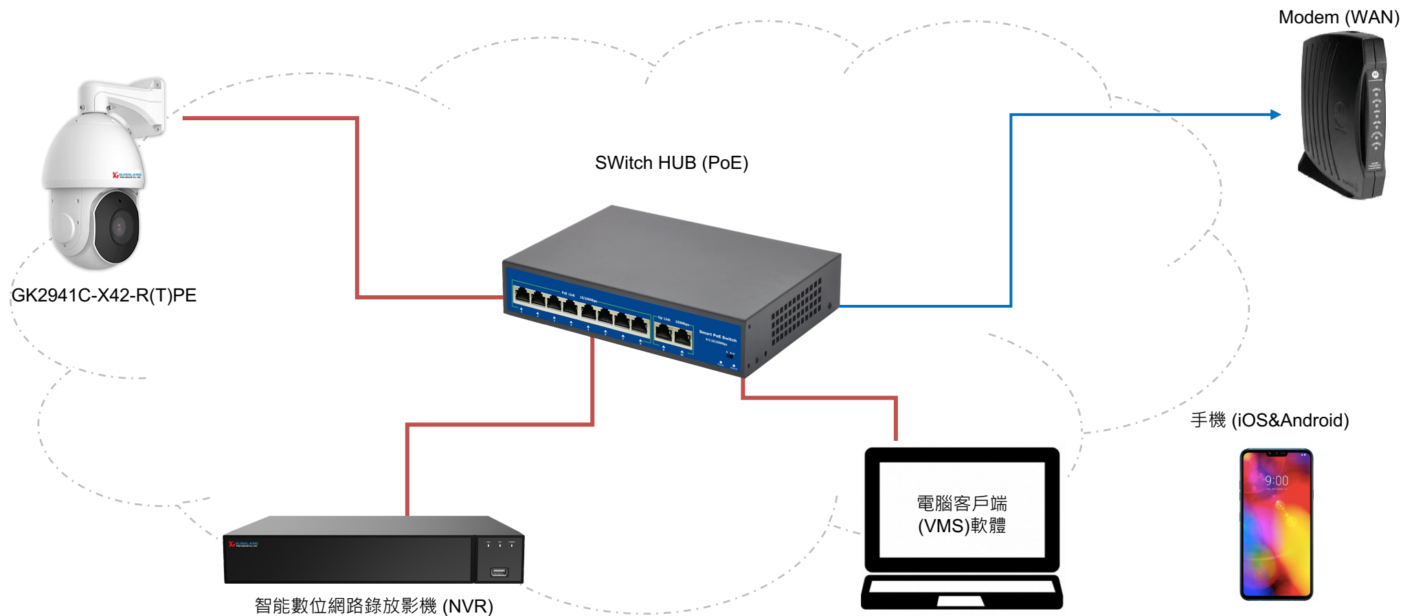
AI 42X Speed Dome Network Camera | Infrastructure
