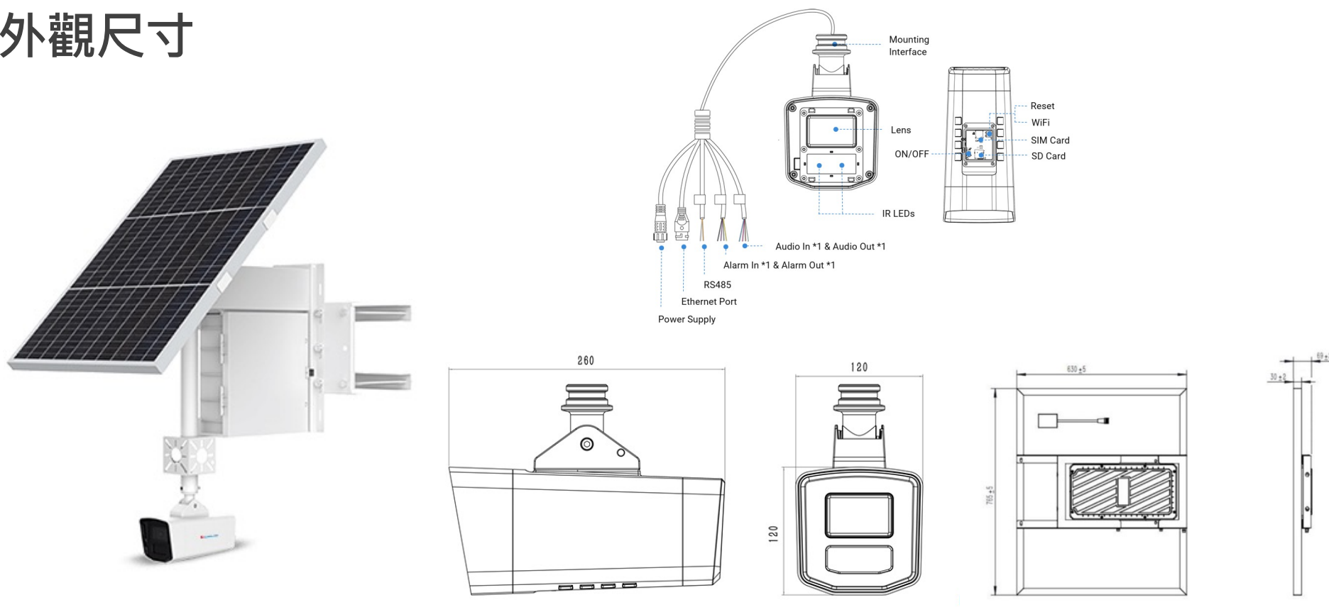
4G Solar-powered ANPR Camera | Dimensions
