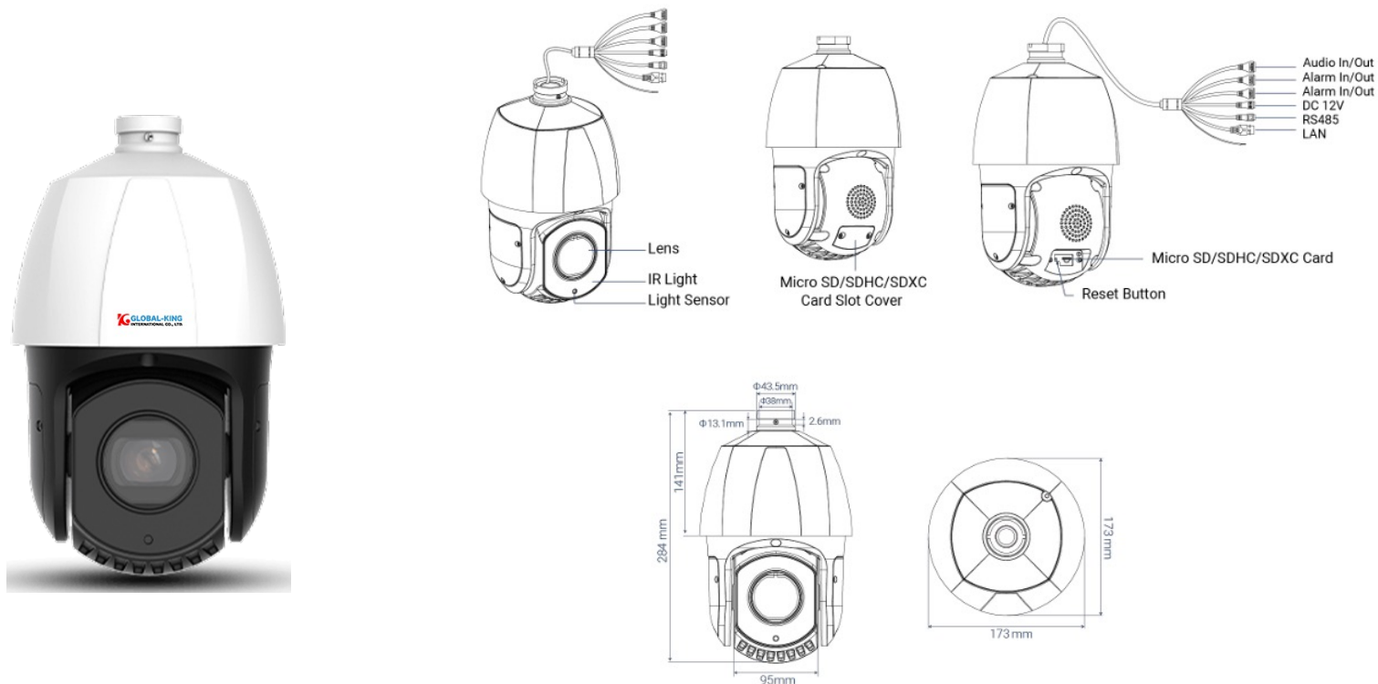
AI 5-inch 25X Speed Dome Network Camera | Dimensions
