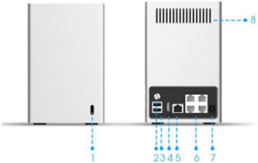
1. LED Indicator 2. Power Button 3. USB 4. HDMI 5. LAN 6. PoE Port 1/2/3/4 7. Power 8. Ventilation Hole
