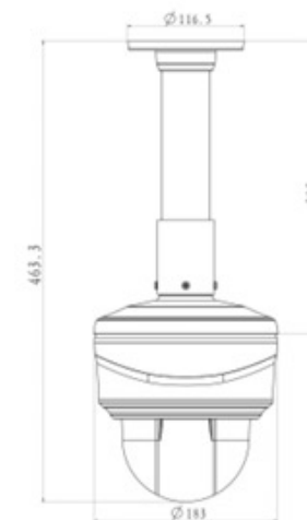
AI 12X PTZ Dome Network Camera | Dimensions
