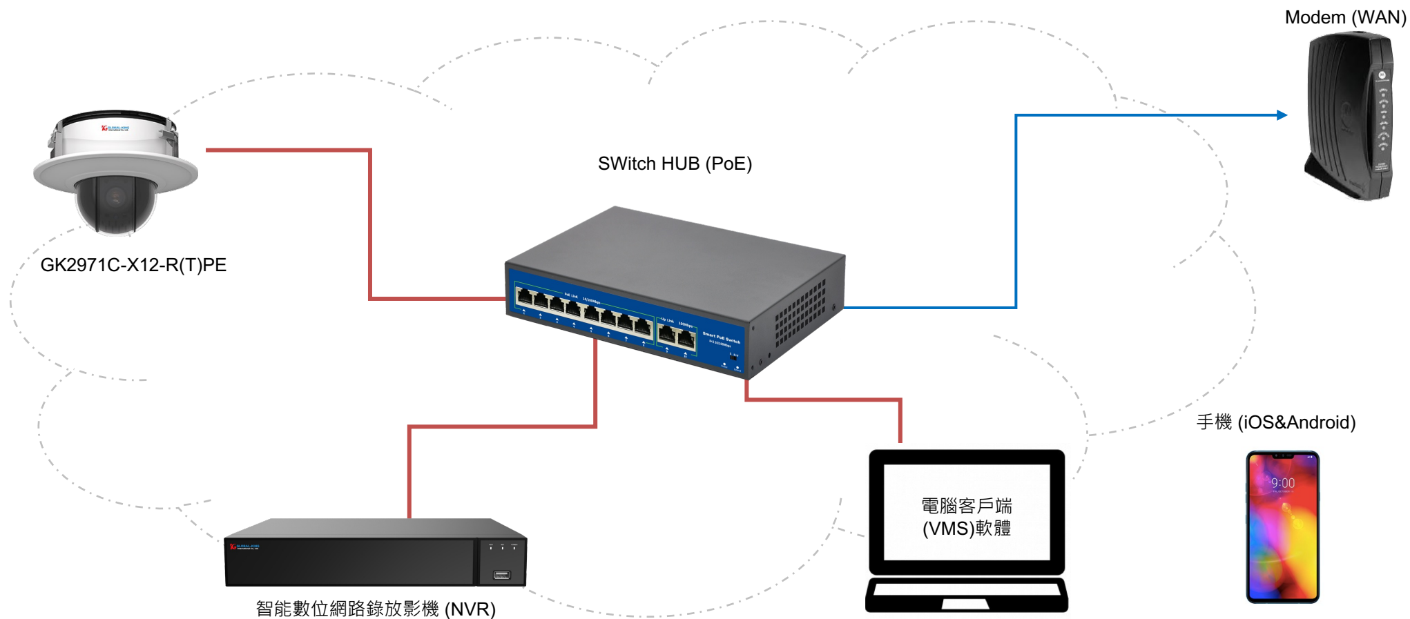
AI 12X PTZ Dome Network Camera | Infrastructure
