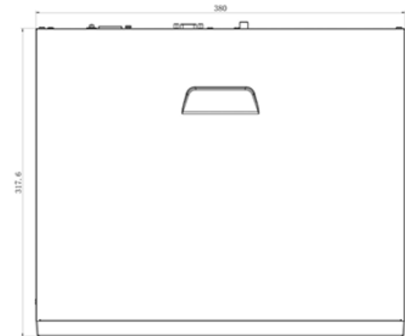
4K Pro NVR 5000 Series | Dimensions
